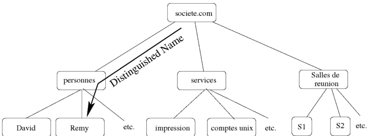
FIGURE 11.2: Exemple de Distinguished Name dn:cn=Remy, ou=personnes, dc=societe, dc=com .
