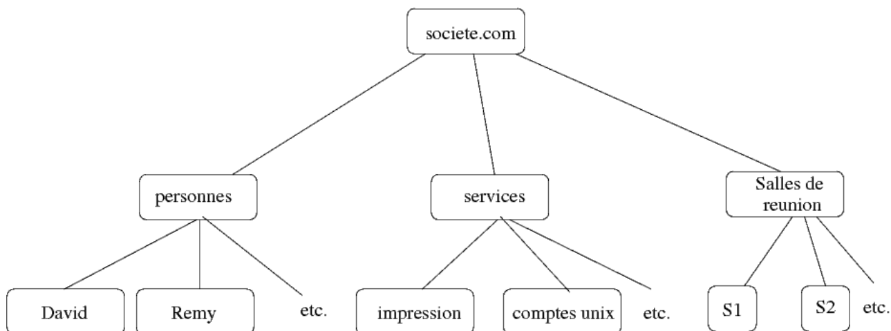
FIGURE 11.1: Exemple de Directory Information Tree (DIT)
